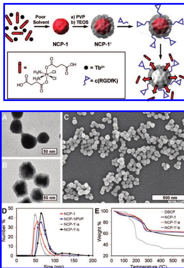
Figure 1. (A) TEM micrograph for as-synthesized NCP-1 . (B) TEM and (C) SEM micrographs for NCP-1'-b . (D) DLS curves for NCP-1 , PVP-functionalized NCP-1 , and NCP-1' . (E) TGA curves for DSCP, NCP-1 , and NCP-1' .
